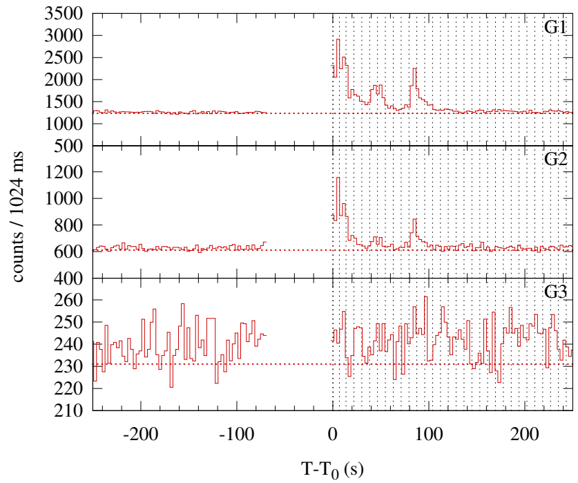
Konus-WIND S2 SOL2000-03-02T16:09 (C2.6) T 0 = 58162.103 s UT (16:09:22.103)
