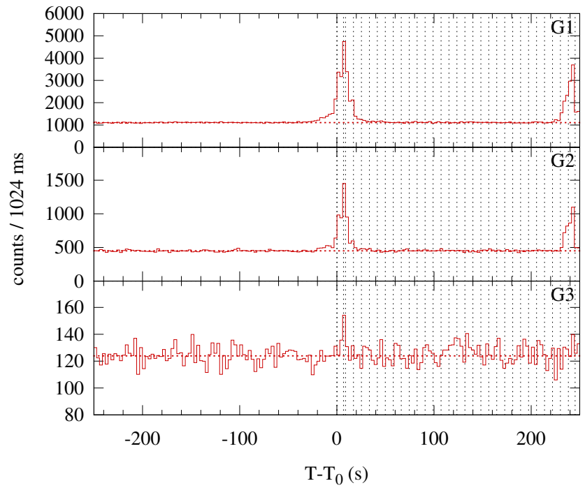
Konus-WIND S2 SOL2000-03-05T15:25 (C3.0) T 0 = 55552.662 s UT (15:25:52.662)
