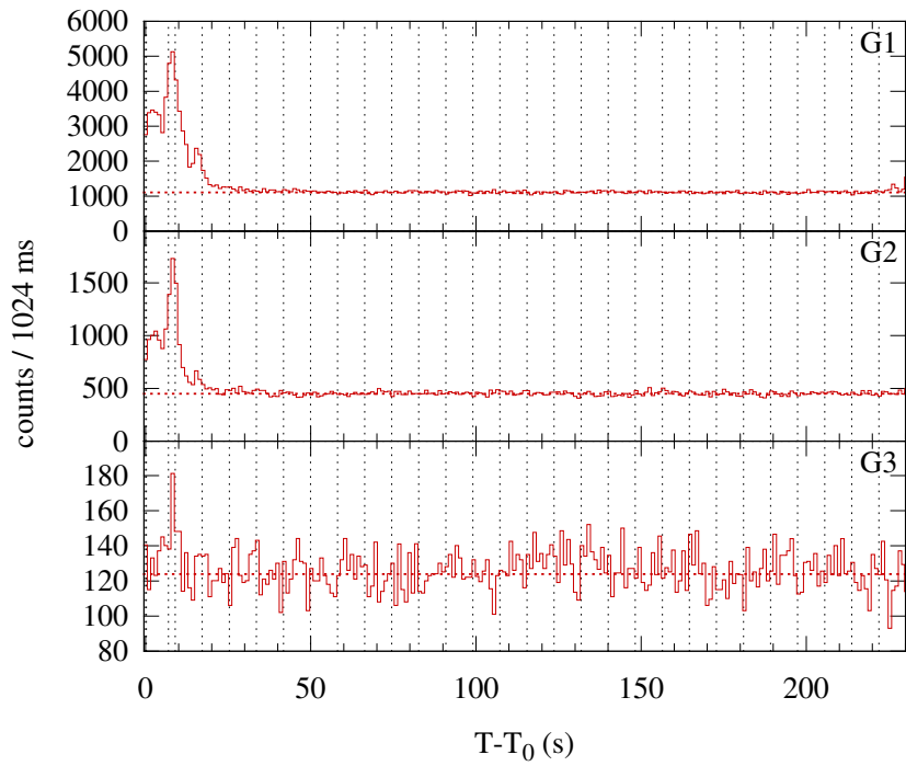
Konus-WIND S2 SOL2000-03-05T15:25 (C3.0) T 0 = 55552.662 s UT (15:25:52.662)
