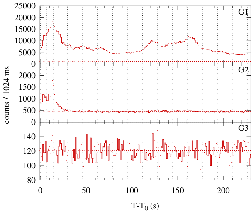
Konus-WIND S2 SOL2000-03-12T23:33 (M3.6) T_0 = 84807.922 s UT (23:33:27.922)
