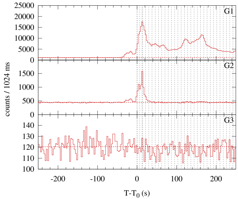
Konus-WIND S2 SOL2000-03-12T23:33 (M3.6) T_0 = 84807.922 s UT (23:33:27.922)
