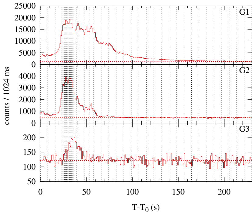
Konus-WIND S2 SOL2000-03-18T23:53 (M3.9) T 0 = 86016.288 s UT (23:53:36.288)
