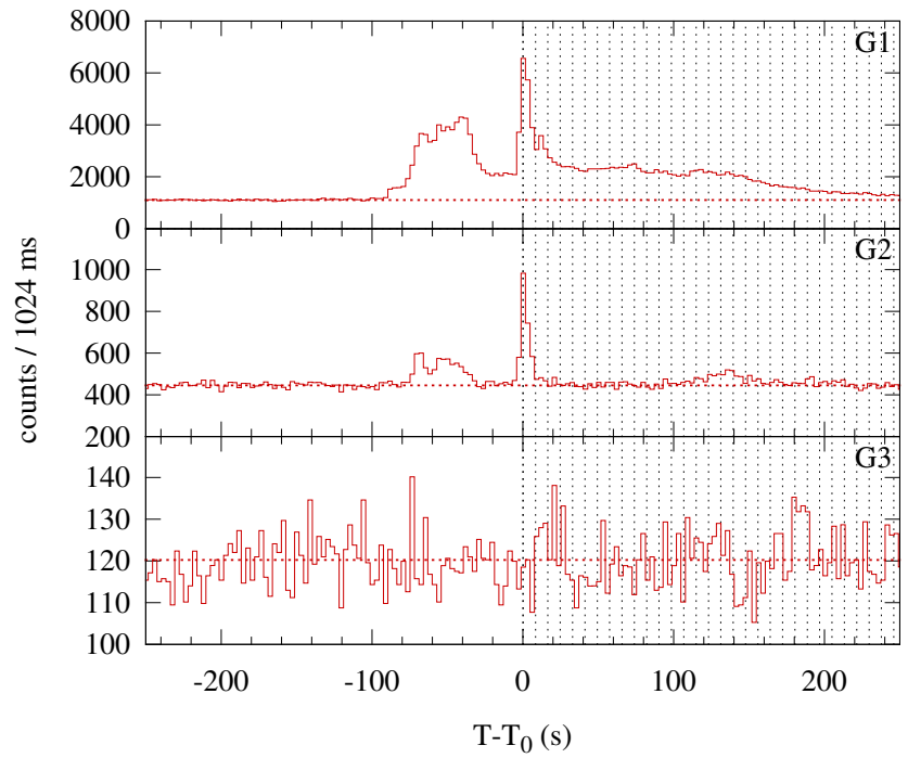
Konus-WIND S2 SOL2000-03-20T16:41 (M2.4) T 0 = 60115.872 s UT (16:41:55.872)
