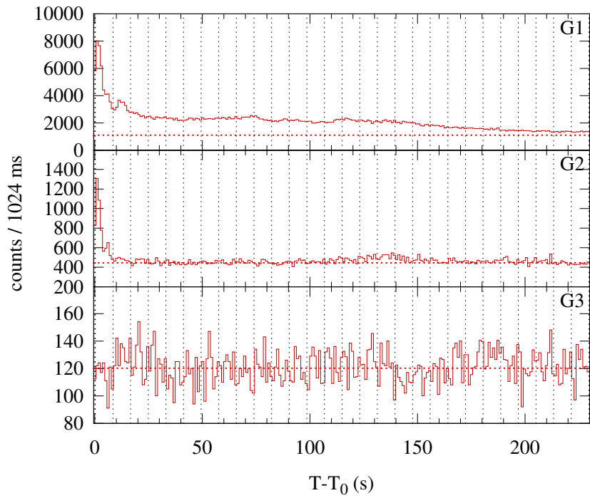
Konus-WIND S2 SOL2000-03-20T16:41 (M2.4) T 0 = 60115.872 s UT (16:41:55.872)
