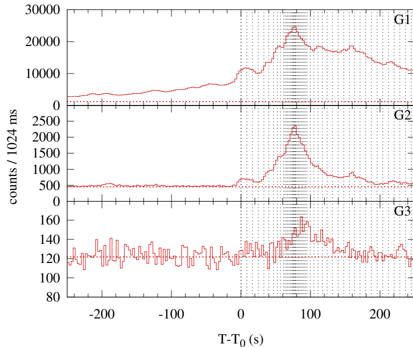
Konus-WIND S2 SOL2000-03-22T18:42 (X1.1) T 0 = 67331.524 s UT (18:42:11.524)
