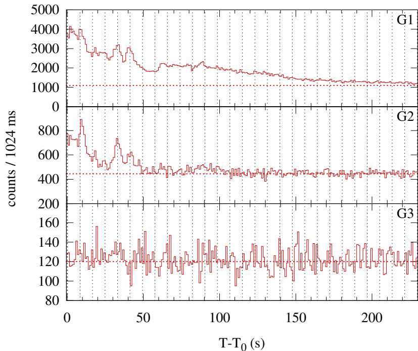
Konus-WIND S2 SOL2000-03-31T13:15 (M1.8) T_0 = 47736.104 s UT (13:15:36.104)
