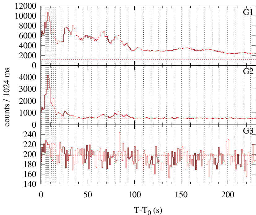
Konus-WIND S2 SOL2000-05-16T15:48 (M3.2) T_0 = 56929.93 s UT (15:48:49.93)
