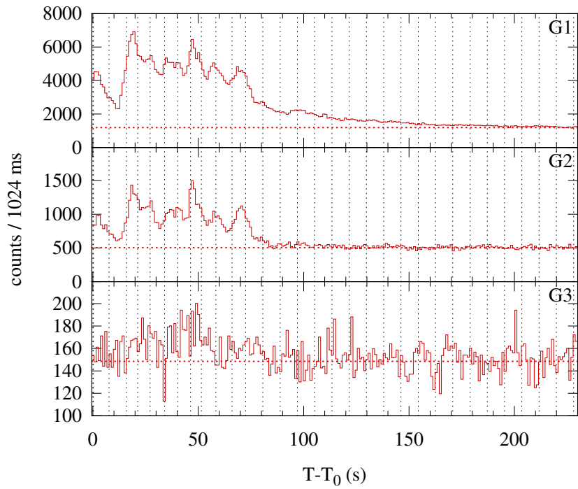
Konus-WIND S2 SOL2000-05-18T15:55 (M2.7) T_0 = 57342.559 s UT (15:55:42.559)
