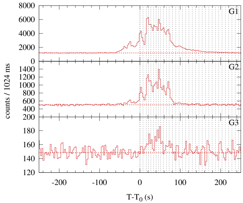
Konus-WIND S2 SOL2000-05-18T15:55 (M2.7) T_0 = 57342.559 s UT (15:55:42.559)
