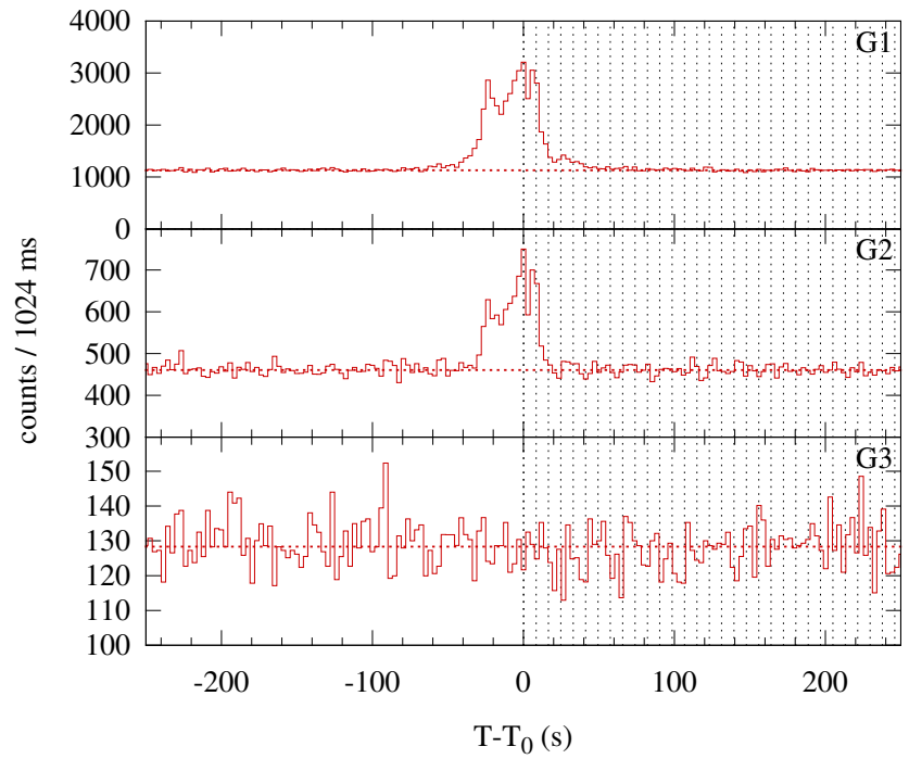
Konus-WIND S2 SOL2000-05-20T20:20 (C2.1) T_0 = 73205.469 s UT (20:20:05.469)
