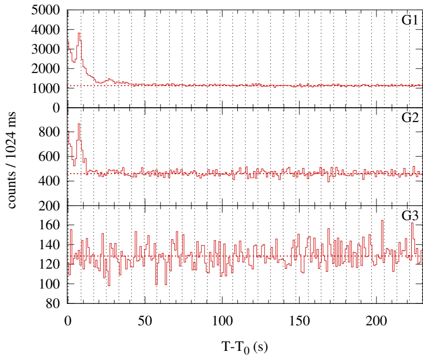
Konus-WIND S2 SOL2000-05-20T20:20 (C2.1) T_0 = 73205.469 s UT (20:20:05.469)
