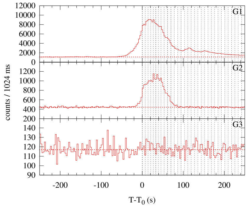
Konus-WIND S2 SOL2000-06-01T06:11 (M2.5) T 0 = 22303.677 s UT (06:11:43.677)
