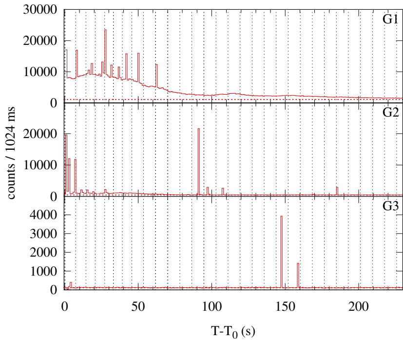
Konus-WIND S2 SOL2000-06-01T06:11 (M2.5) T 0 = 22303.677 s UT (06:11:43.677)
