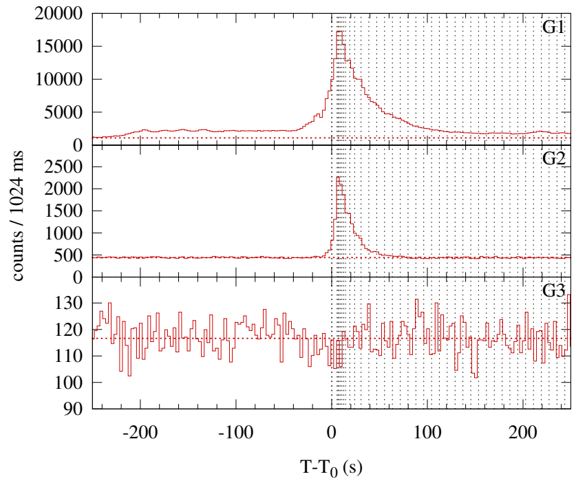
Konus-WIND S2 SOL2000-06-02T19:22 (M7.6) T 0 = 69726.847 s UT (19:22:06.847)
