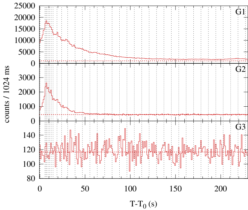
Konus-WIND S2 SOL2000-06-02T19:22 (M7.6) T 0 = 69726.847 s UT (19:22:06.847)
