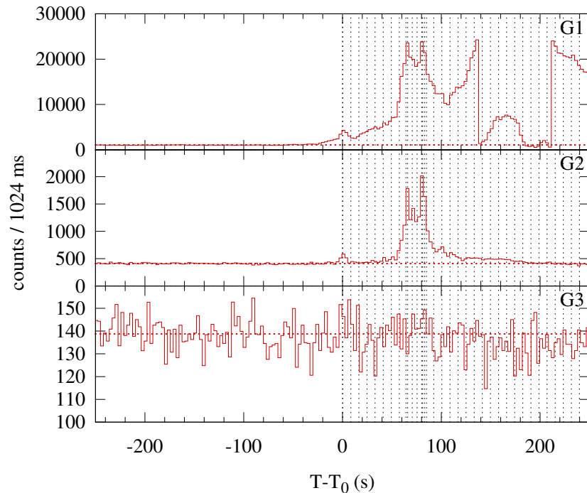
Konus-WIND S1 SOL2000-06-06T13:30 (X1.1) T_0 = 48649.589 s UT (13:30:49.589)
