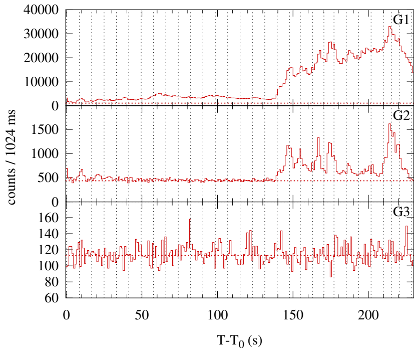
Konus-WIND S2 SOL2000-06-06T15:01 (X2.3) T_0 = 54092.86 s UT (15:01:32.86)
