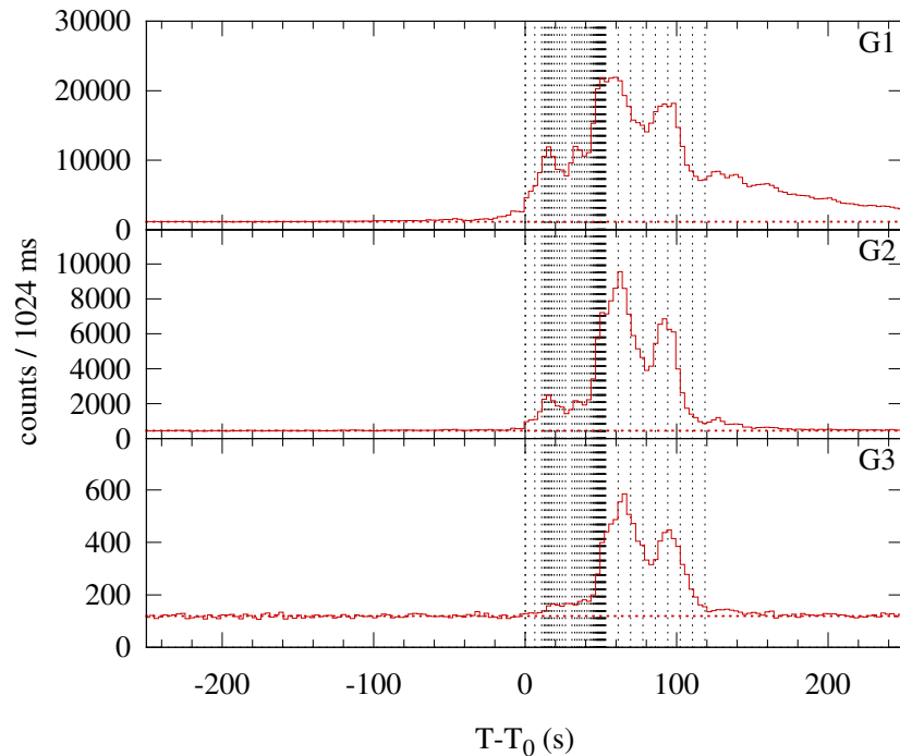
Konus-WIND S2 SOL2000-06-18T01:55 (X1.0) T_0 = 6956.545 s UT (01:55:56.545)
