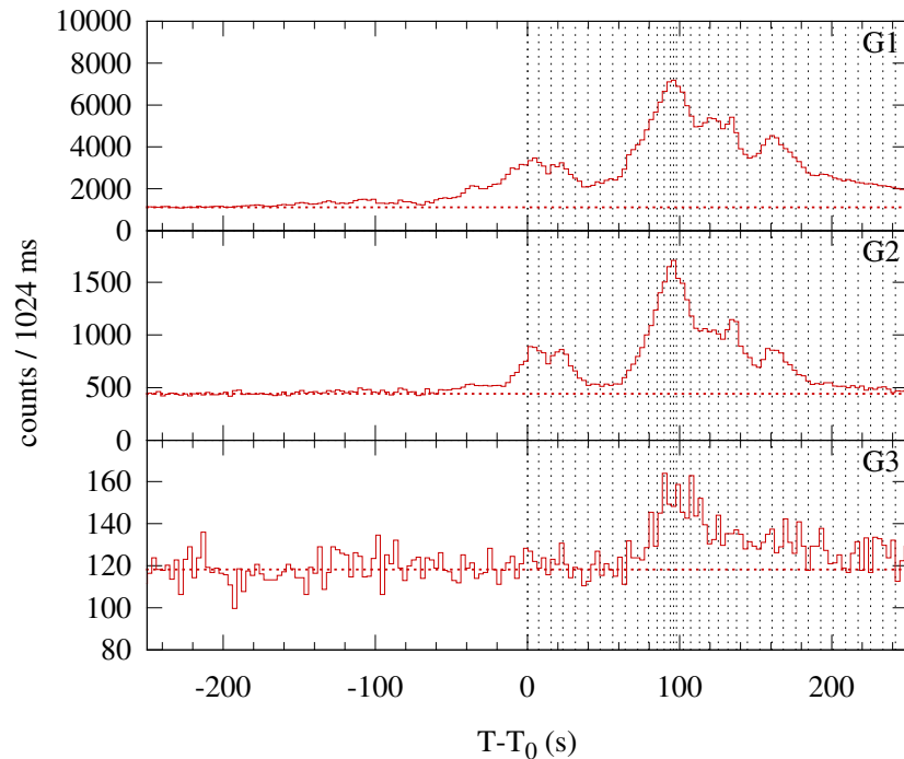
Konus-WIND S2 SOL2000-06-23T14:23 (M3.0) T_0 = 51806.930 s UT (14:23:26.930)
