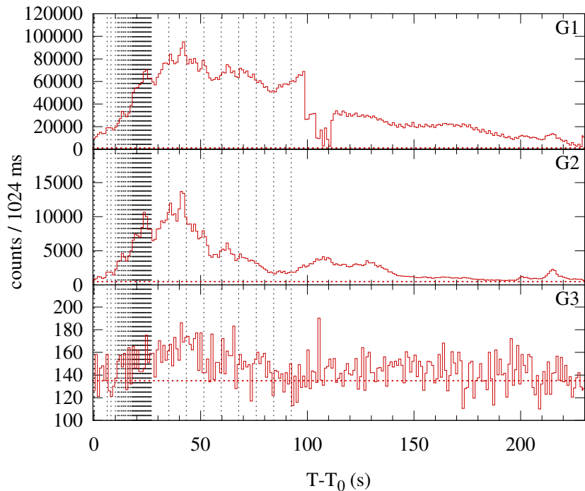
Konus-WIND S2 SOL2000-07-12T10:30 (X1.9) T_0 = 37838.899 s UT (10:30:38.899)
