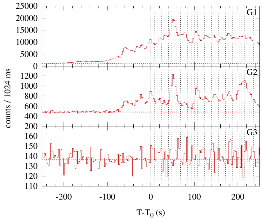
Konus-WIND S2 SOL2000-07-12T18:44 (M5.7) T_0 = 67449.965 s UT (18:44:09.965)
