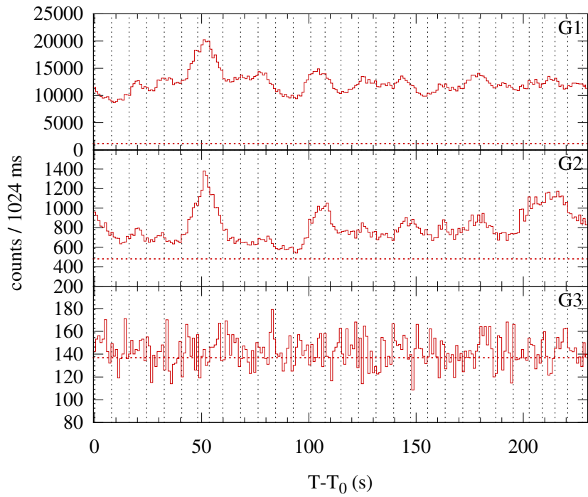
Konus-WIND S2 SOL2000-07-12T18:44 (M5.7) T_0 = 67449.965 s UT (18:44:09.965)
