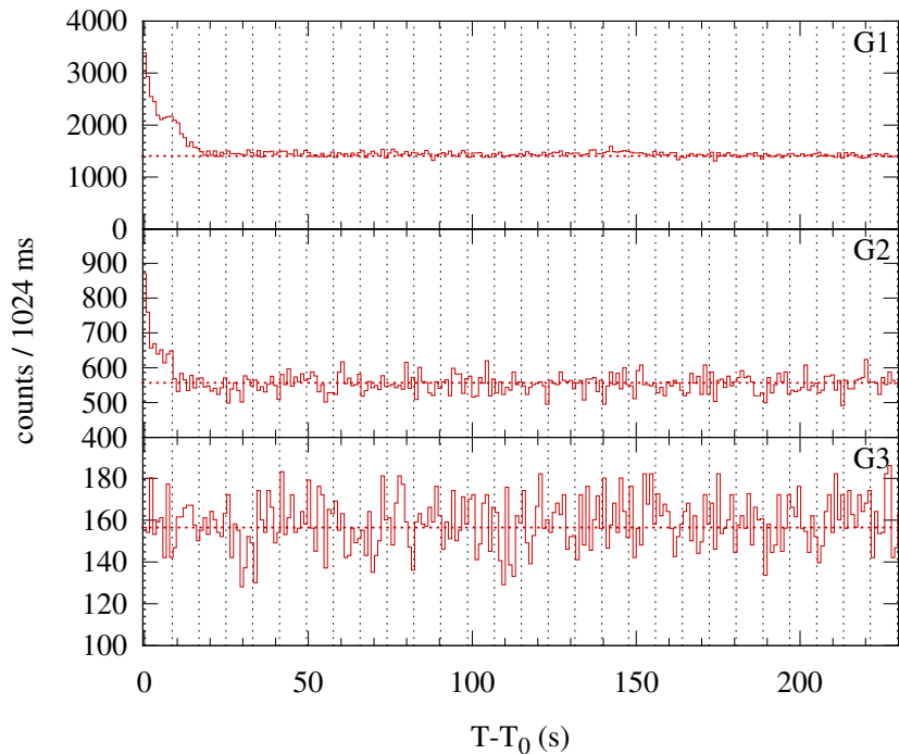
Konus-WIND S2 SOL2000-07-13T06:11 (C7.1) T_0 = 22273.83 s UT (06:11:13.83)
