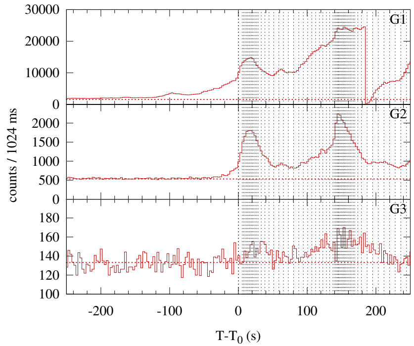
Konus-WIND S2 SOL2000-07-14T10:12 (X5.7) T_0 = 36756.893 s UT (10:12:36.893)
