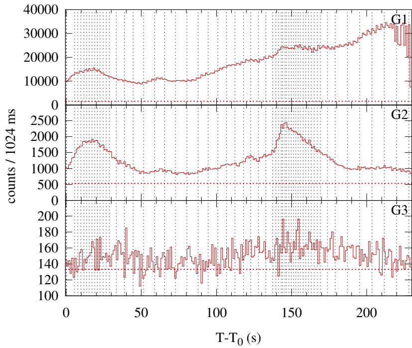
Konus-WIND S2 SOL2000-07-14T10:12 (X5.7) T_0 = 36756.893 s UT (10:12:36.893)
