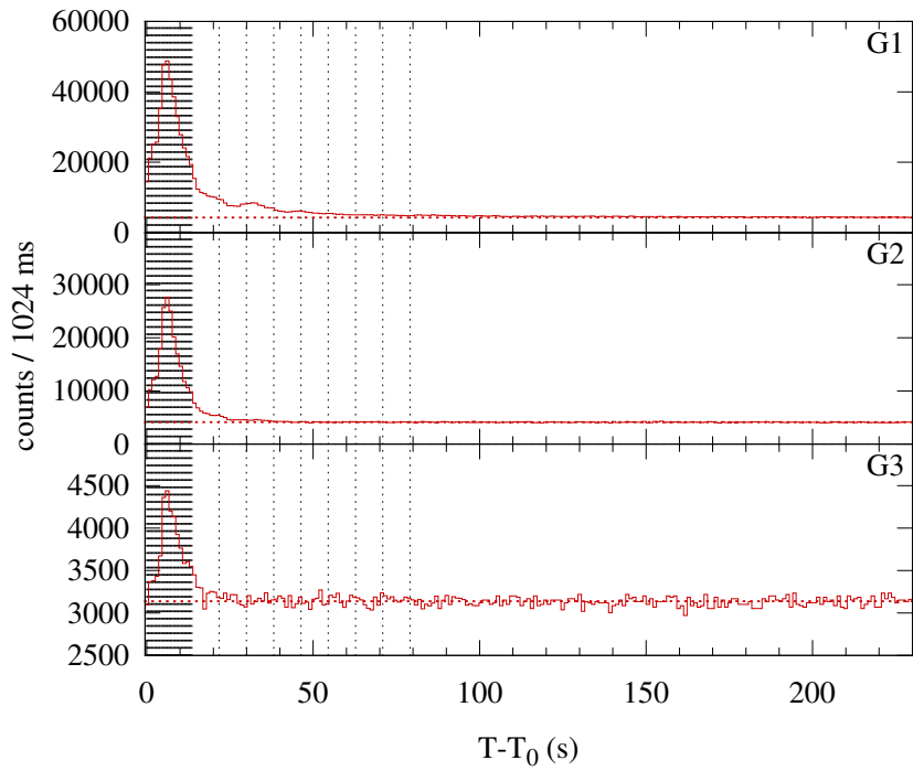
Konus-WIND S2 SOL2000-07-17T20:24 (M2.4) T_0 = 73482.232 s UT (20:24:42.232)
