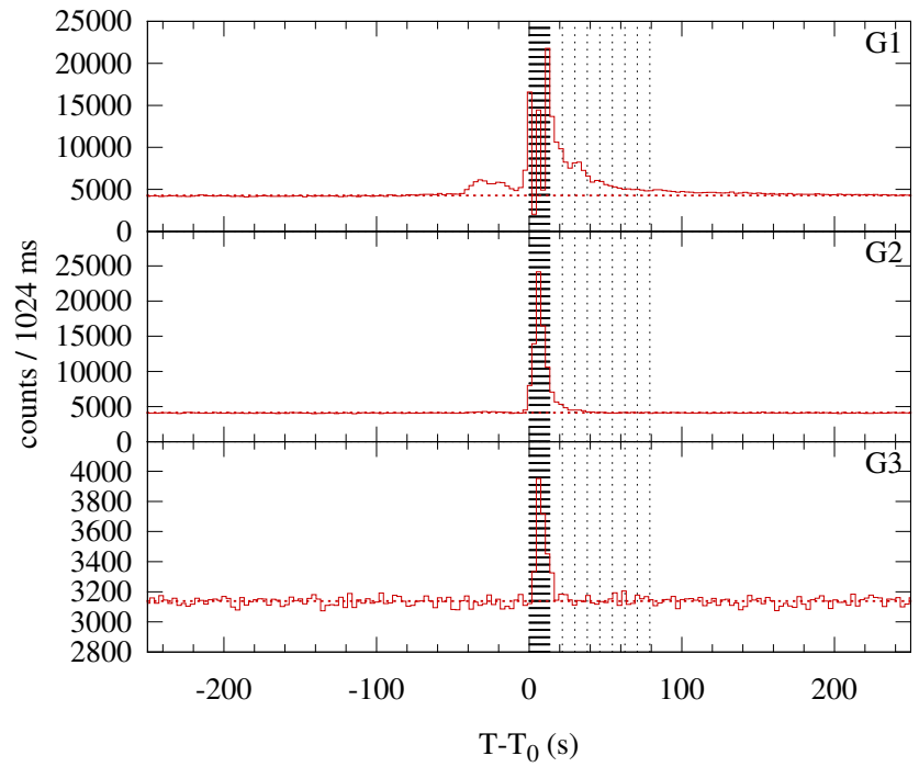
Konus-WIND S2 SOL2000-07-17T20:24 (M2.4) T_0 = 73482.232 s UT (20:24:42.232)
