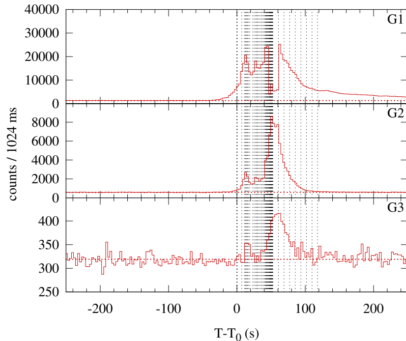
Konus-WIND S2 SOL2000-07-25T02:47 (M8.0) T_0 = 10026.34 s UT (02:47:06.34)
