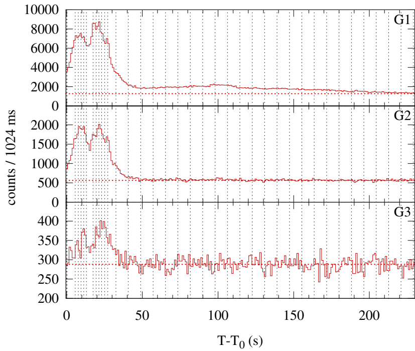
Konus-WIND S2 SOL2000-07-27T04:07 (M2.4) T 0 = 14875.885 s UT (04:07:55.885)
