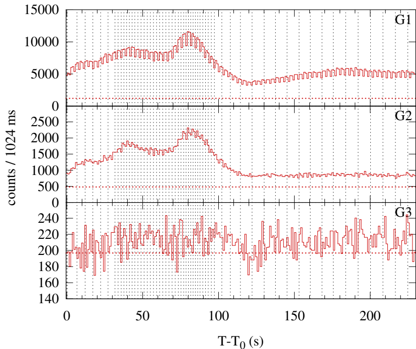
Konus-WIND S1 SOL2000-09-16T04:11 (M5.9) T 0 = 15119.641 s UT (04:11:59.641)
