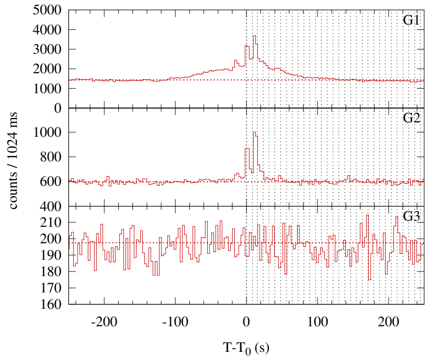
Konus-WIND S2 SOL2000-09-16T14:26 (M3.3) T_0 = 52013.467 s UT (14:26:53.467)
