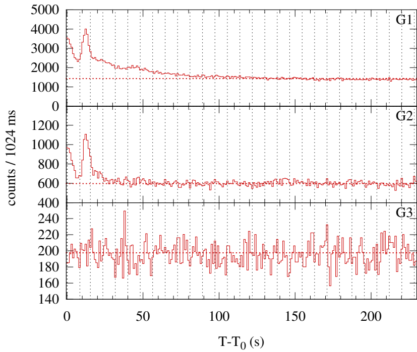
Konus-WIND S2 SOL2000-09-16T14:26 (M3.3) T_0 = 52013.467 s UT (14:26:53.467)
