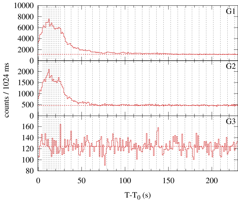
Konus-WIND S2 SOL2000-09-22T09:50 (C4.4) T_0 = 35427.277 s UT (09:50:27.277)
