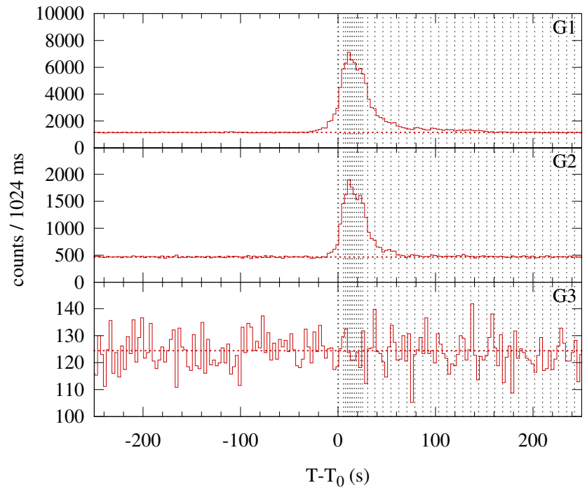
Konus-WIND S2 SOL2000-09-22T09:50 (C4.4) T_0 = 35427.277 s UT (09:50:27.277)
