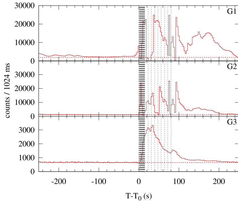
Konus-WIND S2 SOL2000-11-24T15:07 (X2.3) T_0 = 54455.657 s UT (15:07:35.657)
