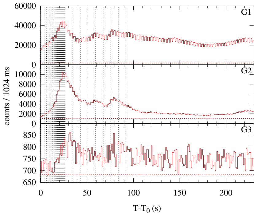
Konus-WIND S1 SOL2000-11-25T18:37 (X1.9) T 0 = 67065.70 s UT (18:37:45.70)
