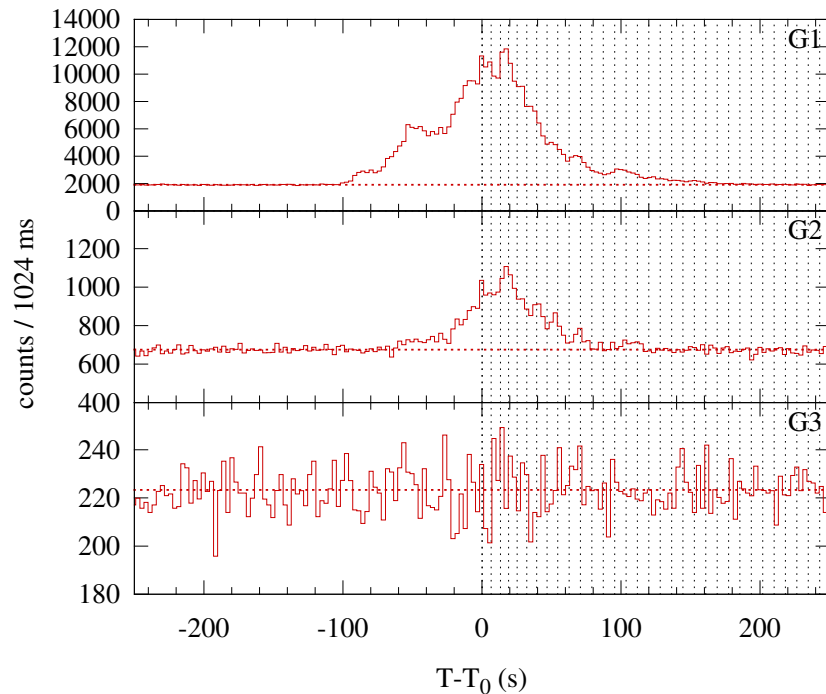
Konus-WIND S2 SOL2002-01-14T01:54 (M1.7) T_0 = 6893.845 s UT (01:54:53.845)
