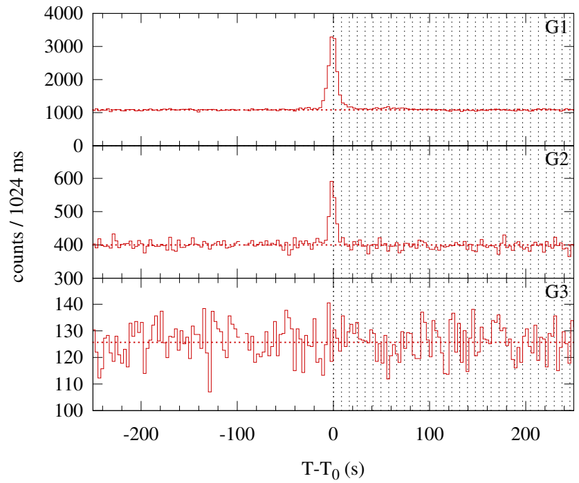
Konus-WIND S2 SOL2002-03-12T19:07 (C2.2) T 0 = 68830.730 s UT (19:07:10.730)
