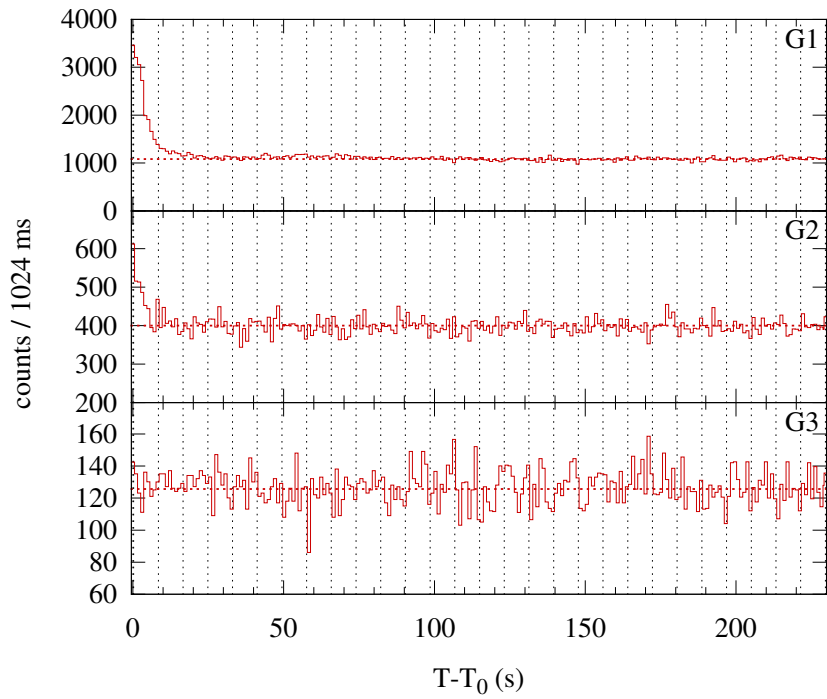
Konus-WIND S2 SOL2002-03-12T19:07 (C2.2) T 0 = 68830.730 s UT (19:07:10.730)
