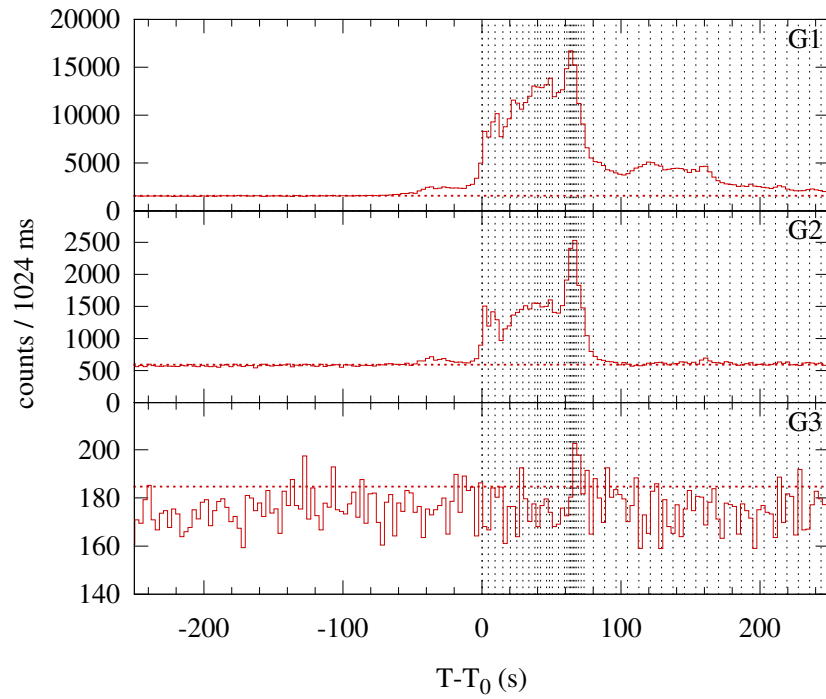
Konus-WIND S2 SOL2002-03-17T19:27 (M4.0) T_0 = 70059.912 s UT (19:27:39.912)
