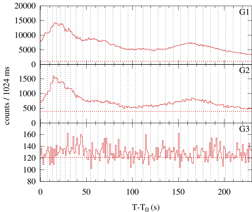
Konus-WIND S2 SOL2002-04-10T12:27 (M8.2) T 0 = 44868.152 s UT (12:27:48.152)
