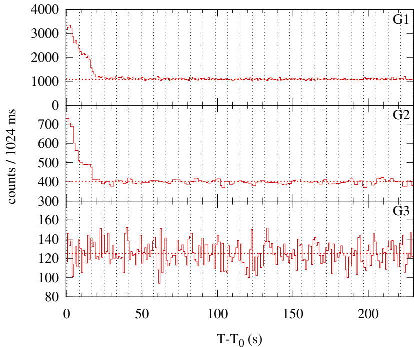
Konus-WIND S2 SOL2002-04-14T22:25 (C7.2) T_0 = 80735.449 s UT (22:25:35.449)
