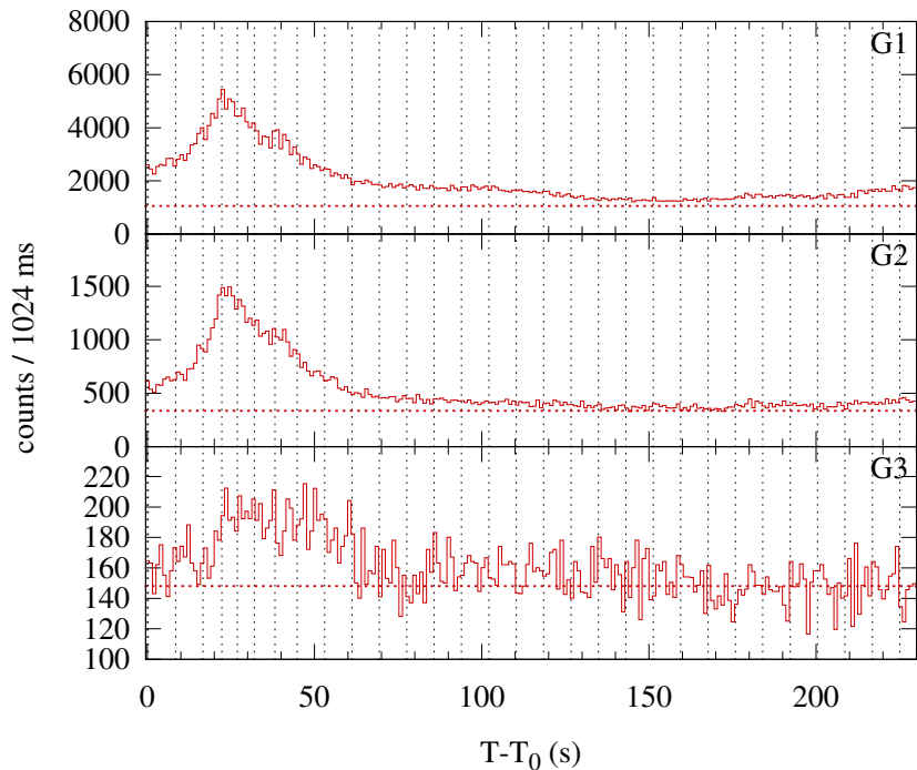
Konus-WIND S1 SOL2002-05-31T00:06 (M2.4) T 0 = 404.306 s UT (00:06:44.306)
