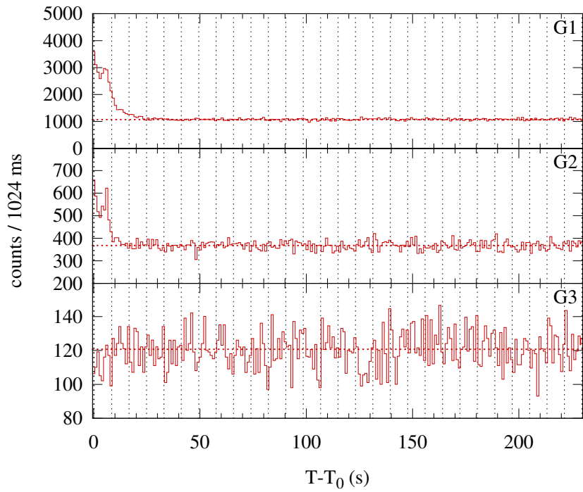
Konus-WIND S2 SOL2002-06-29T09:29 (C2.0) T 0 = 34185.671 s UT (09:29:45.671)
