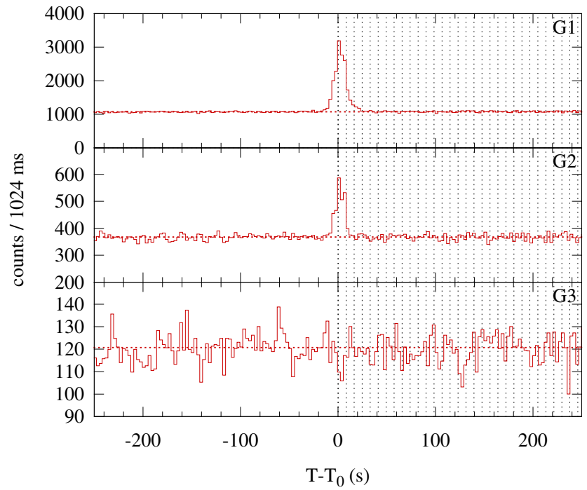
Konus-WIND S2 SOL2002-06-29T09:29 (C2.0) T 0 = 34185.671 s UT (09:29:45.671)
