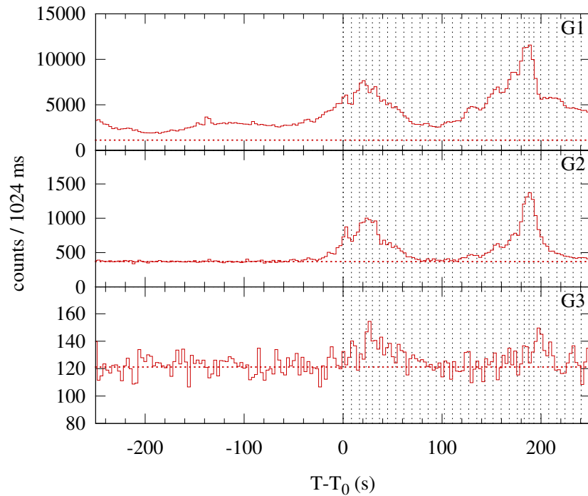
Konus-WIND S2 SOL2002-07-03T20:08 (M5.3) T_0 = 72525.170 s UT (20:08:45.170)
