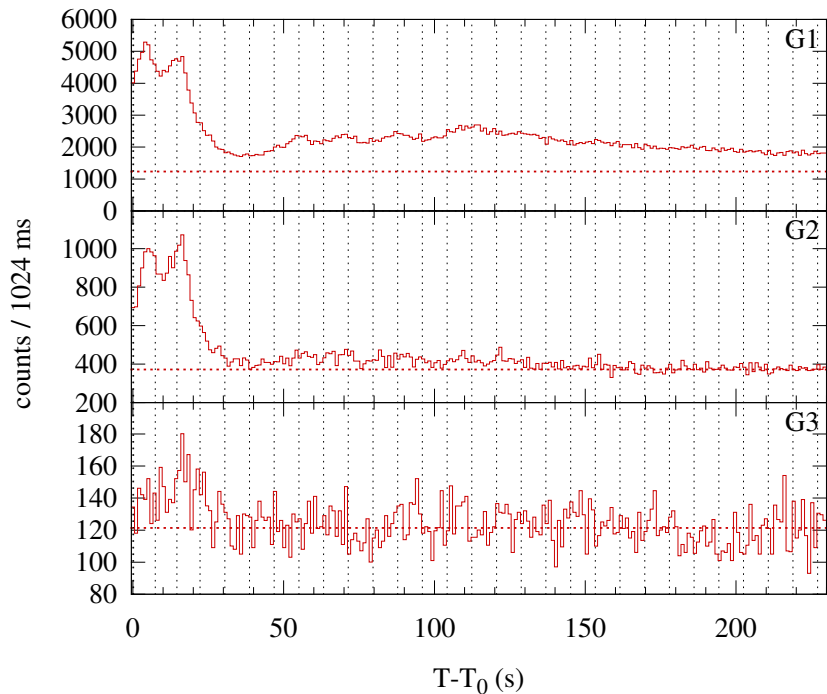
Konus-WIND S2 SOL2002-07-05T13:20 (M3.2) T_0 = 48042.221 s UT (13:20:42.221)
