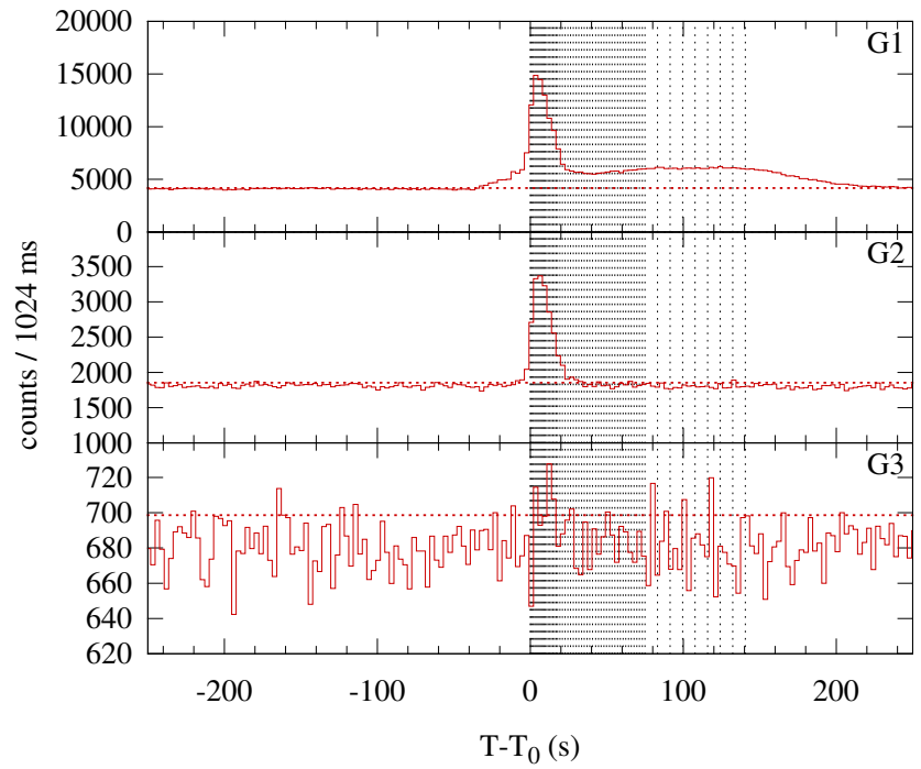
Konus-WIND S2 SOL2002-07-18T03:32 (M2.2) T_0 = 12772.174 s UT (03:32:52.174)
