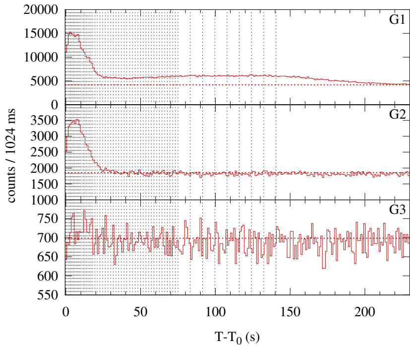
Konus-WIND S2 SOL2002-07-18T03:32 (M2.2) T_0 = 12772.174 s UT (03:32:52.174)
