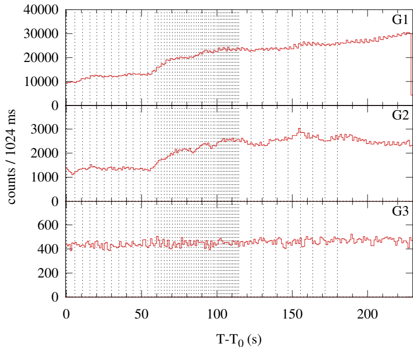
Konus-WIND S2 SOL2002-07-20T21:06 (X3.3) T_0 = 75978.205 s UT (21:06:18.205)
