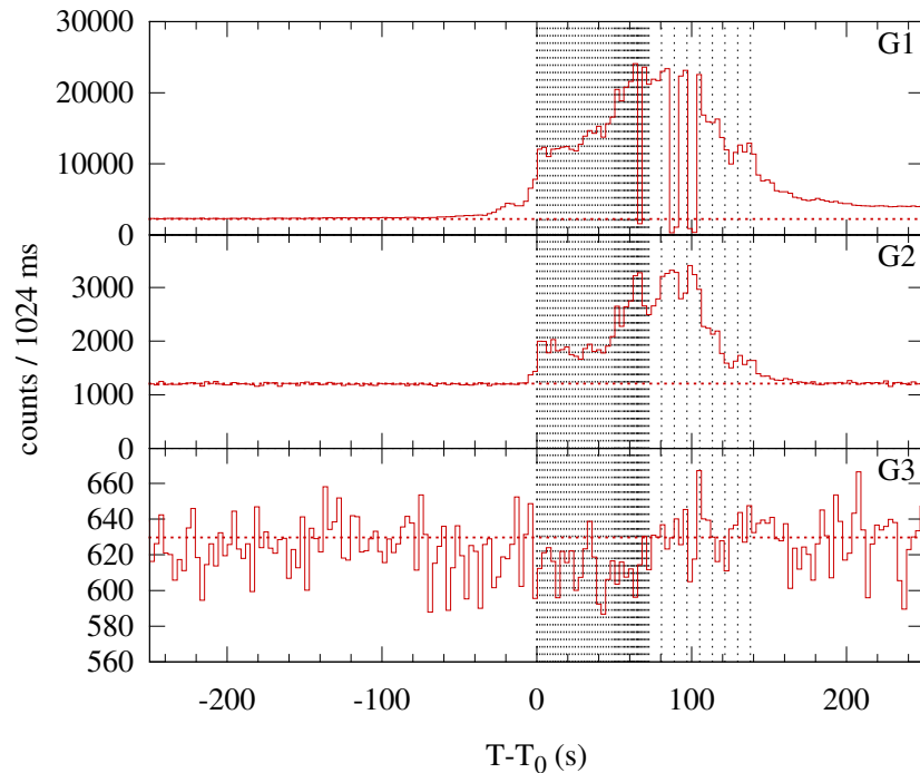
Konus-WIND S1 SOL2002-07-26T22:06 (M5.3) T 0 = 79610.407 s UT (22:06:50.407)
