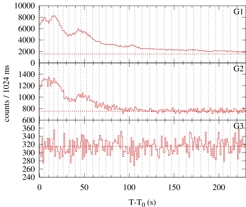
Konus-WIND S2 SOL2002-07-29T02:35 (M4.8) T 0 = 9358.627 s UT (02:35:58.627)
