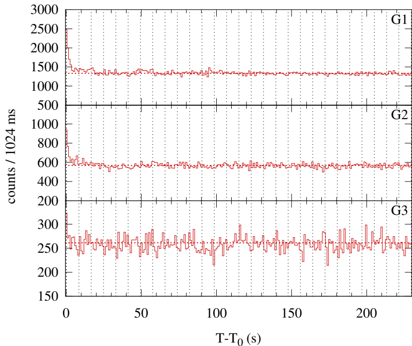
Konus-WIND S1 SOL2002-07-29T17:54 (C3.8) T 0 = 64460.354 s UT (17:54:20.354)
