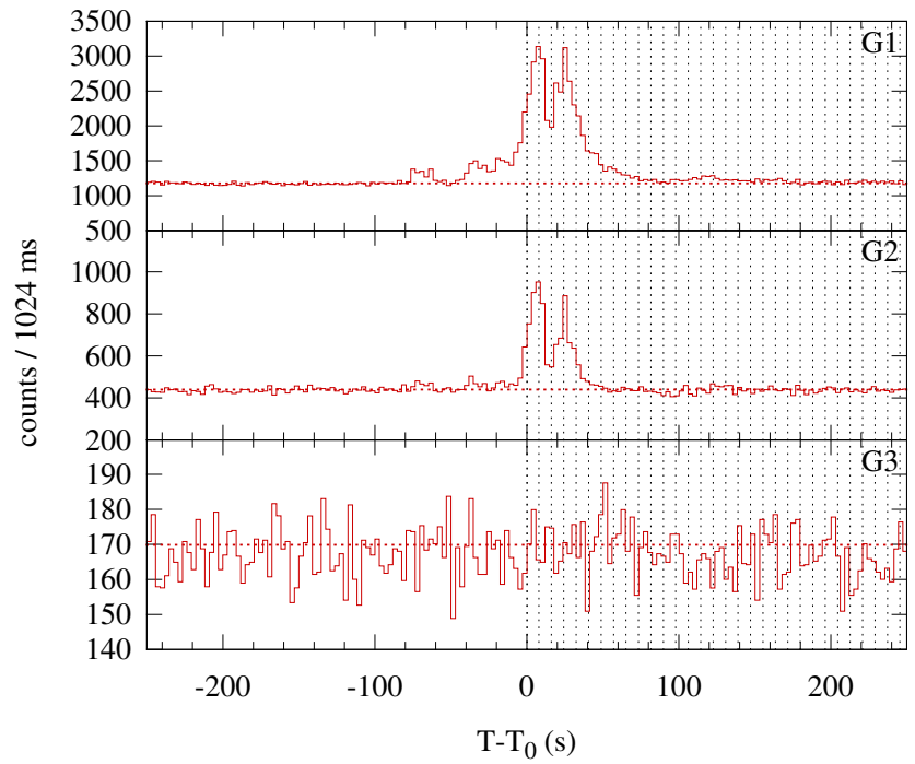
Konus-WIND S2 SOL2002-08-04T07:17 (C7.4) T 0 = 26269.918 s UT (07:17:49.918)
