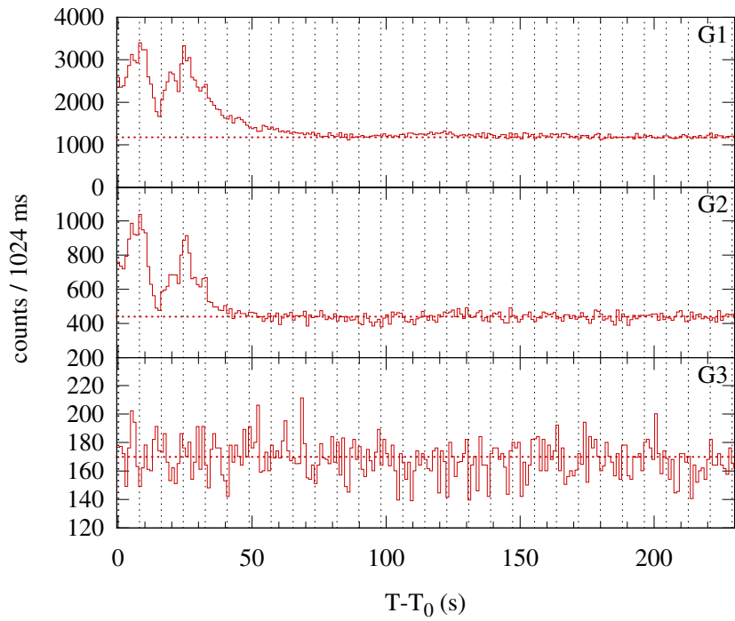
Konus-WIND S2 SOL2002-08-04T07:17 (C7.4) T 0 = 26269.918 s UT (07:17:49.918)
