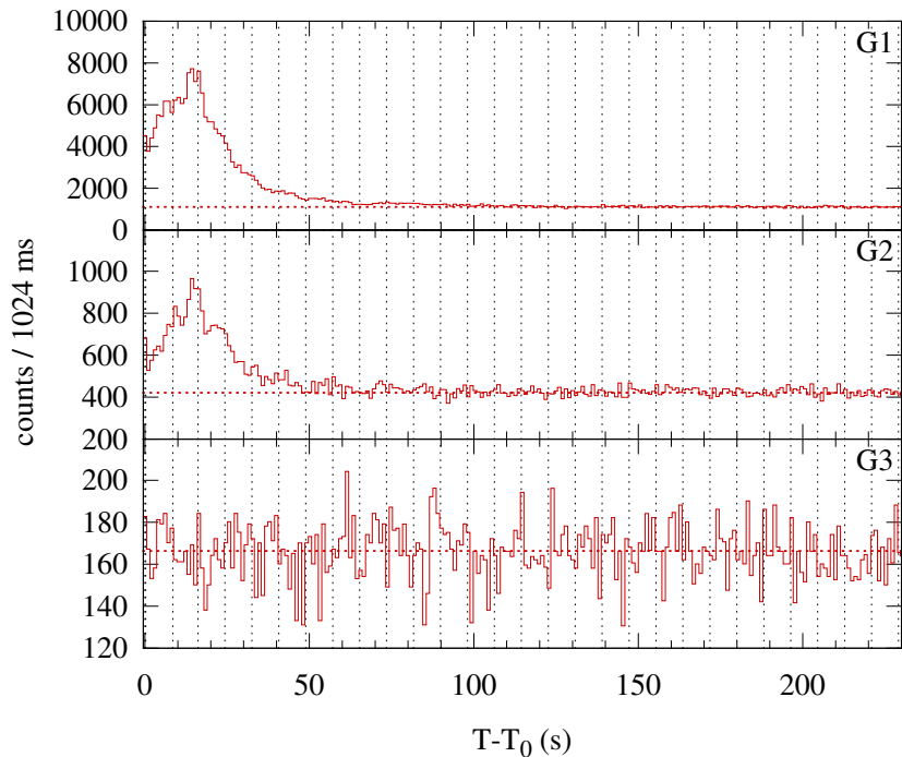
Konus-WIND S2 SOL2002-08-15T06:04 (M1.0) T_0 = 21841.505 s UT (06:04:01.505)
