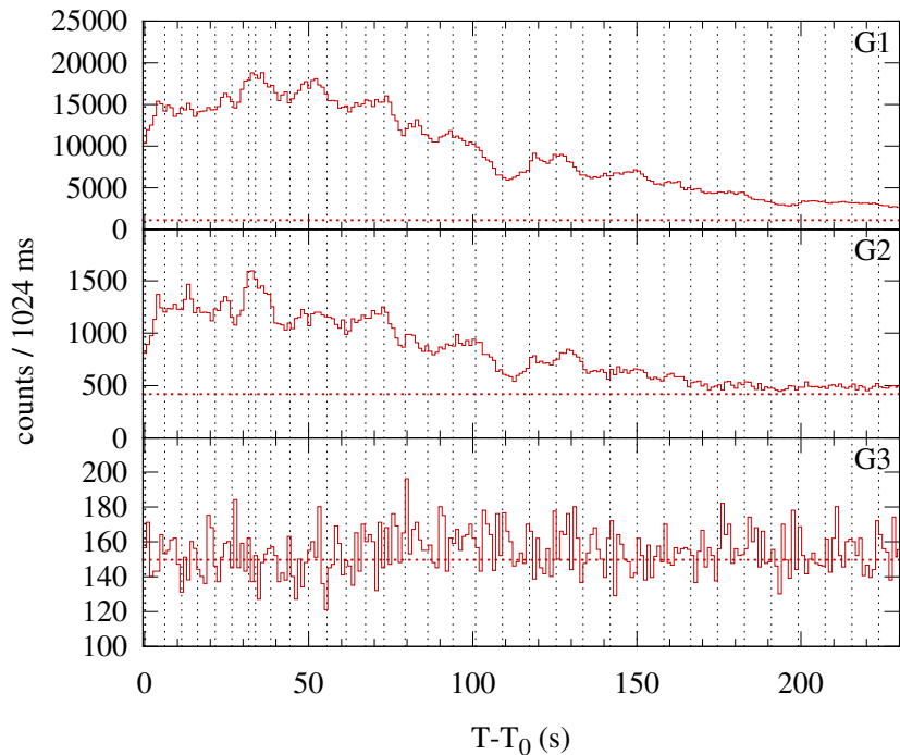
Konus-WIND S2 SOL2002-08-22T01:51 (M5.4) T 0 = 6686.786 s UT (01:51:26.786)
