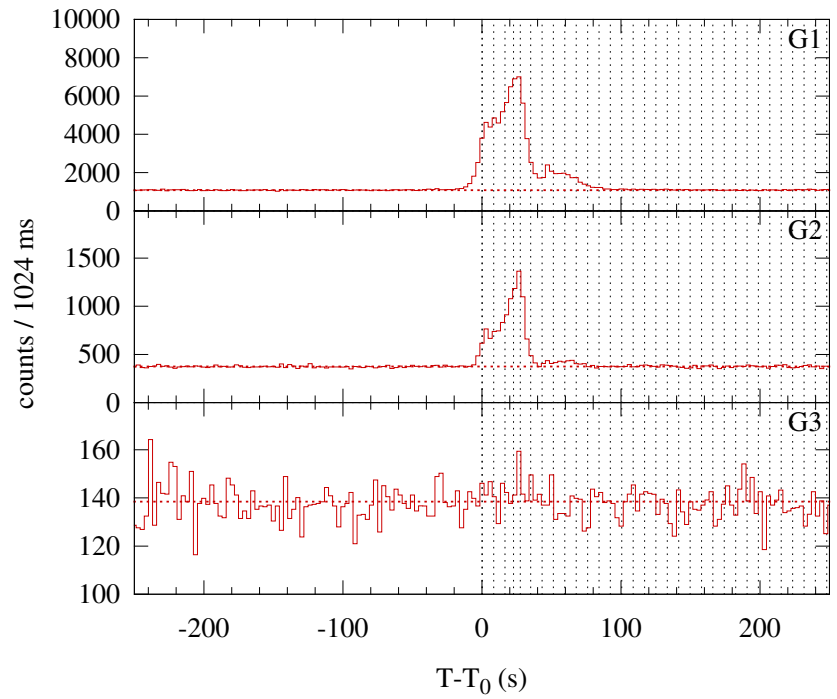
Konus-WIND S2 SOL2002-08-28T10:59 (C5.7) T_0 = 39542.984 s UT (10:59:02.984)
