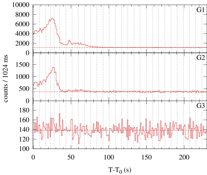
Konus-WIND S2 SOL2002-08-28T10:59 (C5.7) T_0 = 39542.984 s UT (10:59:02.984)
