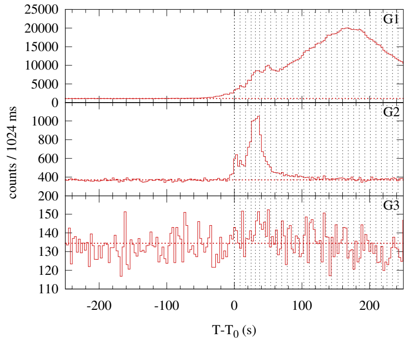
Konus-WIND S2 SOL2002-08-28T18:54 (M4.6) T_0 = 68058.271 s UT (18:54:18.271)
