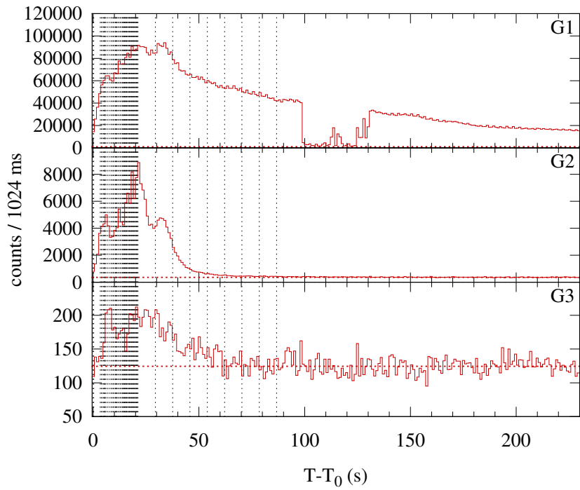
Konus-WIND S2 SOL2002-08-30T13:27 (X1.5) T_0 = 48458.843 s UT (13:27:38.843)
