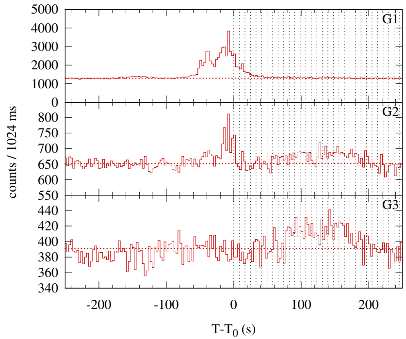
Konus-WIND S2 SOL2002-09-06T16:27 (C9.2) T_0 = 59227.11 s UT (16:27:07.11)
