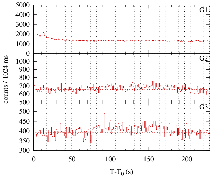
Konus-WIND S2 SOL2002-09-06T16:27 (C9.2) T_0 = 59227.11 s UT (16:27:07.11)
