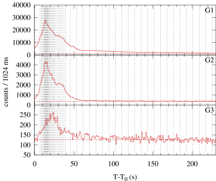
Konus-WIND S2 SOL2002-09-10T14:52 (M2.9) T_0 = 53559.257 s UT (14:52:39.257)
